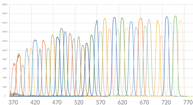
Wavelengths [nm] of the TE292 filters
